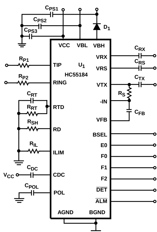
FIGURE 18. HC55184 BASIC APPLICATION CIRCUIT
