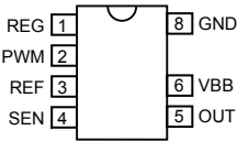
Pin-out Diagram
