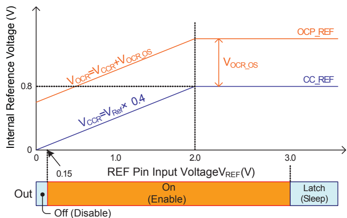
REF Pin Voltage Characteristics
