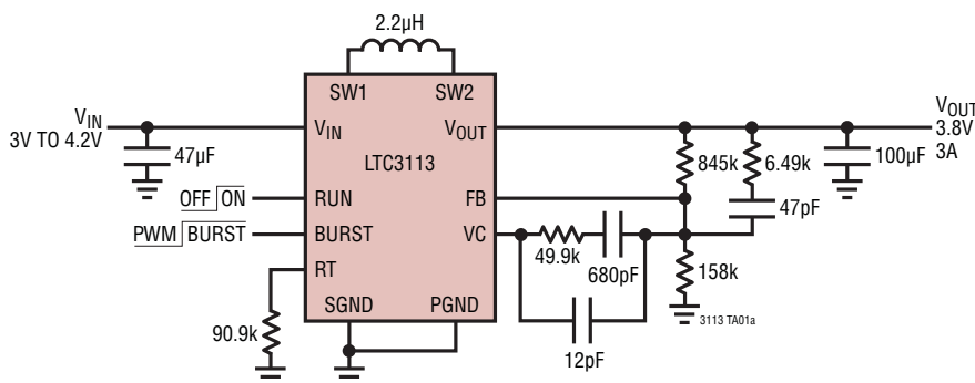
Li-Ion to 3.8V/3A
