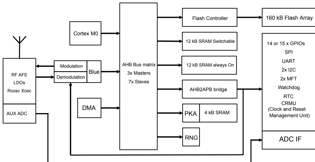
Figure 1. BlueNRG-1 architecture
