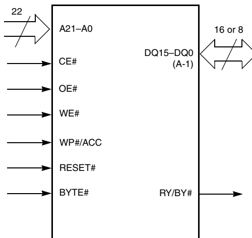
Figure 5.2 S29GL064S Logic Symbol (Models 03, 04)
