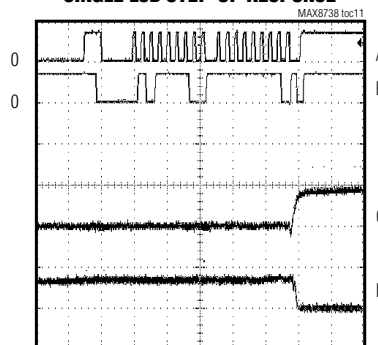
SINGLE LSB STEP-UP RESPONSE
