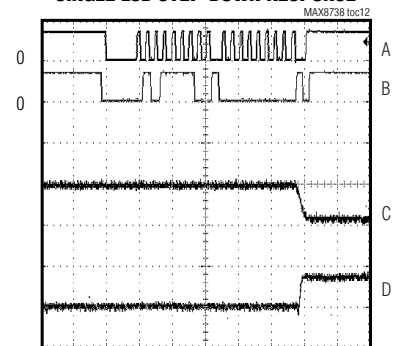
SINGLE LSB STEP-DOWN RESPONSE
