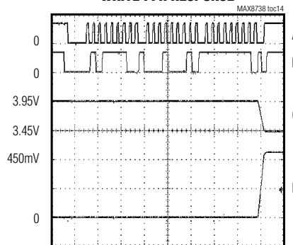
WRITE FFH RESPONSE
