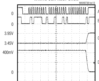
WRITE 00H RESPONSE
