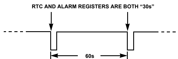
FIGURE 16. \overline{\text{IRQ}}/\text{F}_{\text{OUT}} WAVEFORM
