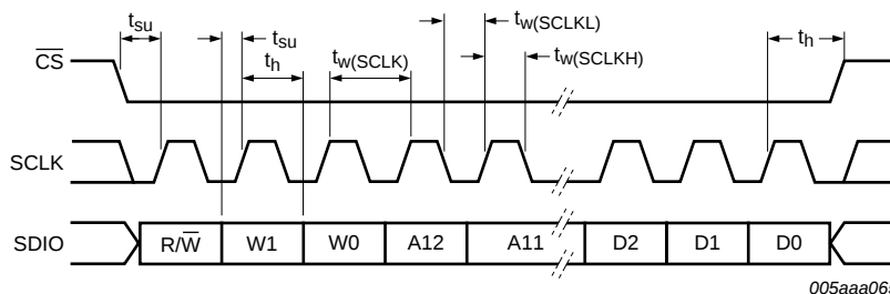
Fig 6. SPI timing
