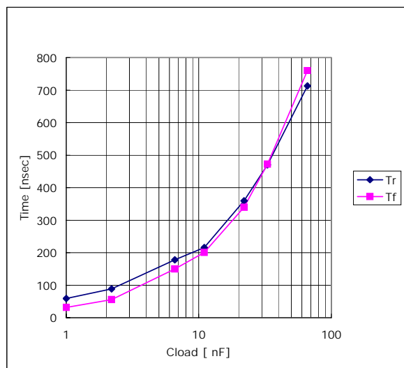
Figure 4. Cload vs. Tr &amp; Tf
