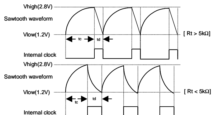
Figure 15. Sawtooth &amp; Clock Waveform
