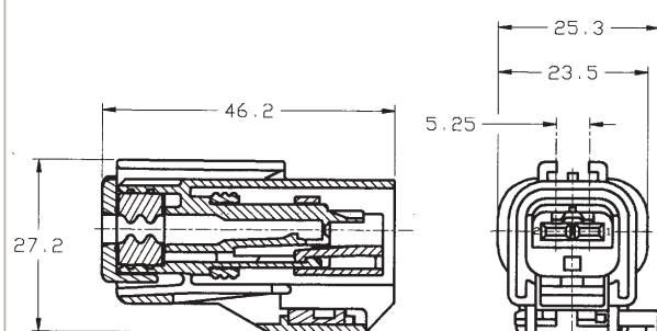
2 way female housing
