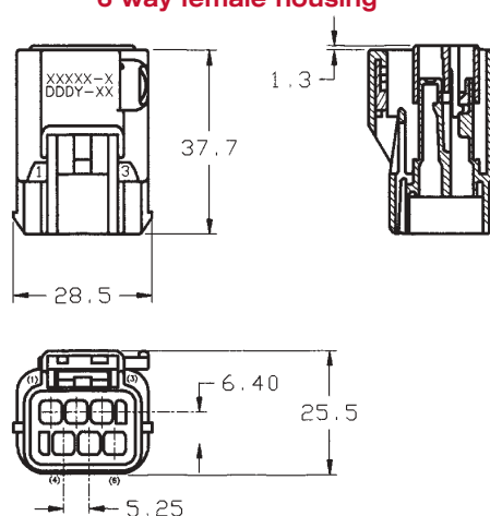
6 way female housing
