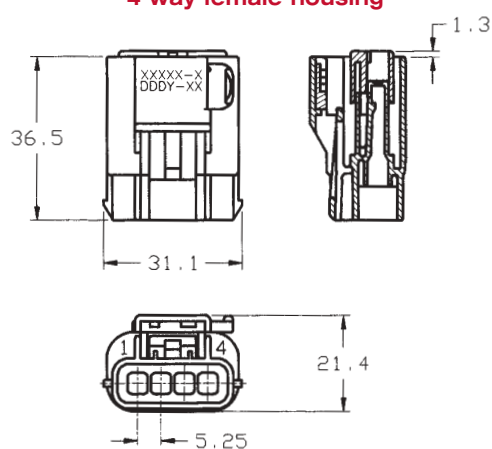
4 way female housing
