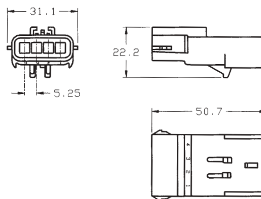
4 way male housing
