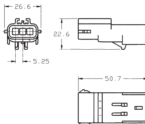
3 way male housing
