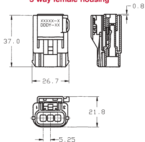
3 way female housing
