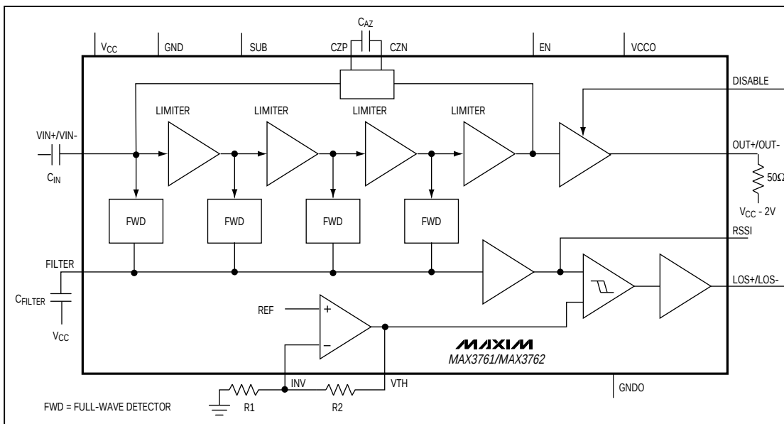
Figure 1. Functional Diagram
