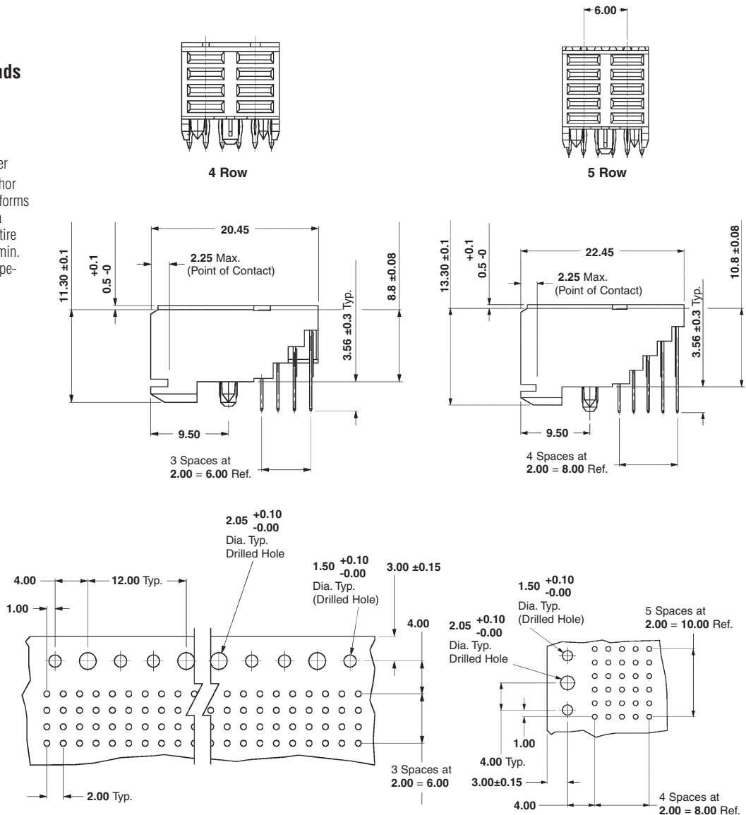
Recommended PC Board Hole Layout per IPC-D-300, Type II, Class C (Component Side)
