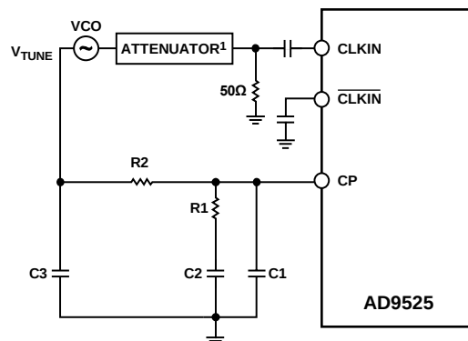
1 VCO MANUFACTURERS RECOMMEND EITHER A T OR PI ATTENUATOR TO PREVENT VCO PULLING. REFER TO MANUFACTURER'S RECOMMENDATION
