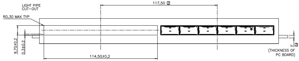
RECOMMENDED SINGLE SIDE MOUNTING BEZEL DESIGN
