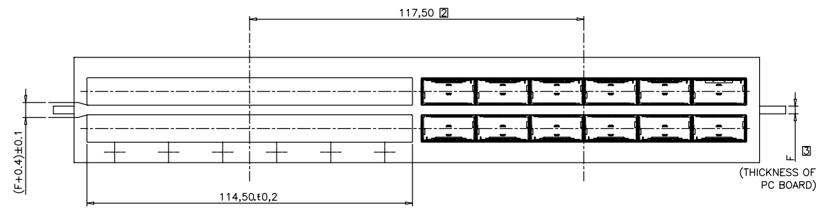
RECOMMENDED DOUBLE SIDE MOUNTING BEZEL DESIGN
