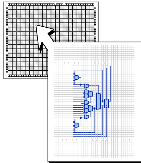
FIGURE 1. 320 Logic Cells
