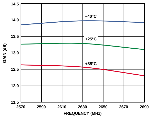
Figure 17. Gain vs. Frequency and Temperature, 2570 MHz to 2690 MHz
