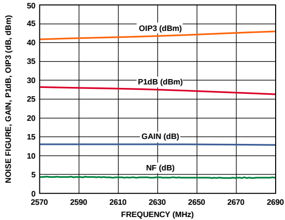
Figure 16. Gain, P1dB, OIP3, and Noise Figure vs. Frequency, 2570 MHz to 2690 MHz
