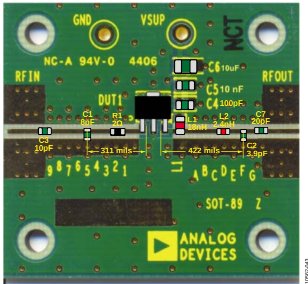
Figure 42. Evaluation Board Layout and Component Placement, 728 MHz to 768 MHz Operation
