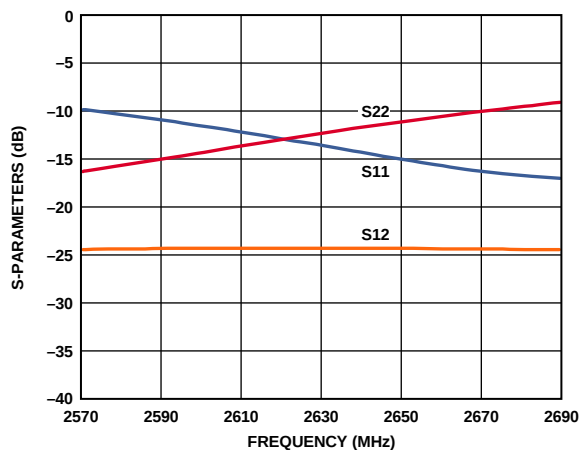
Figure 18. Input Return Loss (S11), Output Return Loss (S22), and Reverse Isolation (S12) vs. Frequency, 2570 MHz to 2690 MHz
