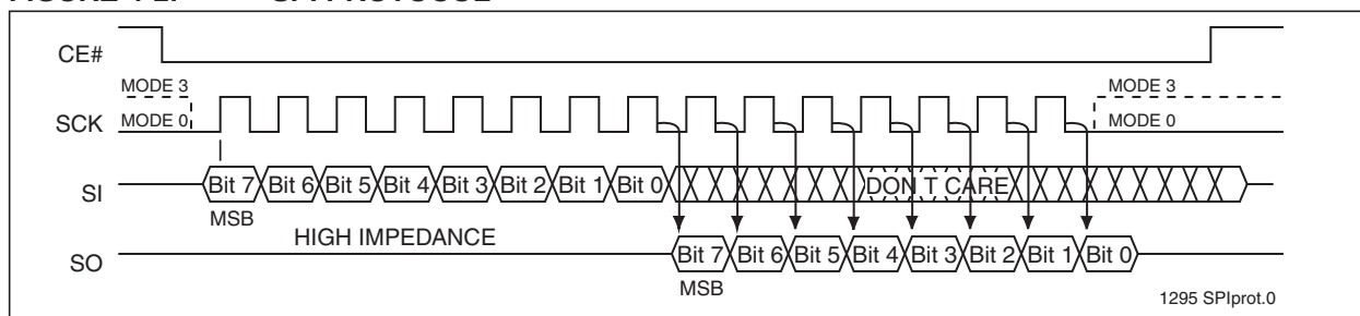
FIGURE 4-1: SPI PROTOCOL
