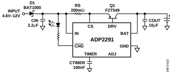
Figure 22. Typical Application Circuit
