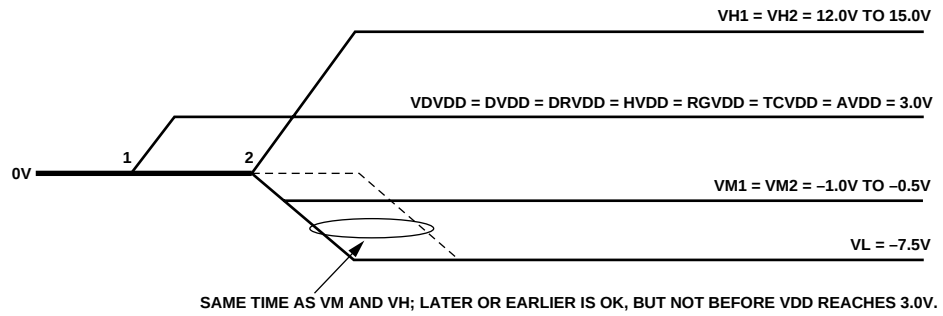
Figure 65. Power-Up Sequence
