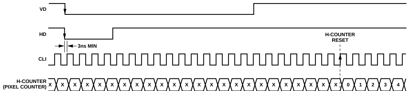
Figure 68. SYNC Timing to Synchronize AD9925 with External Timing
