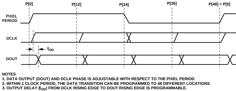
Figure 21. Digital Output Phase Adjustment
