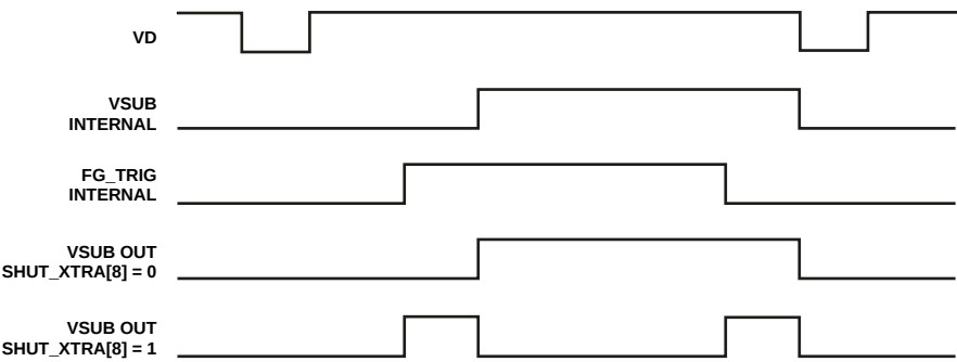
Figure 54. Combining FG_TRIG and VSUB to Create Four Toggle Positions for VSUB Output
