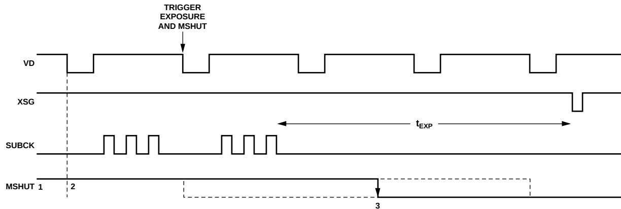
Figure 48. VSUB Programmability
