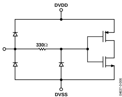
Figure 6. Digital Inputs
