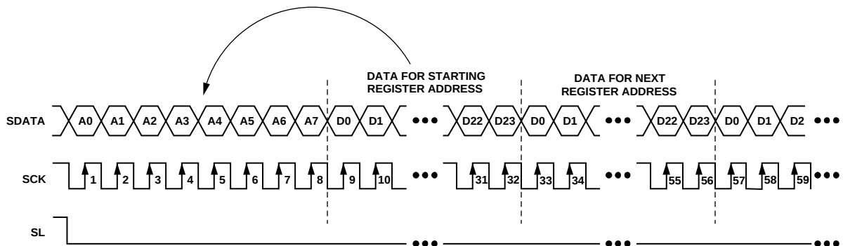
Figure 74. Serial Write Operation
