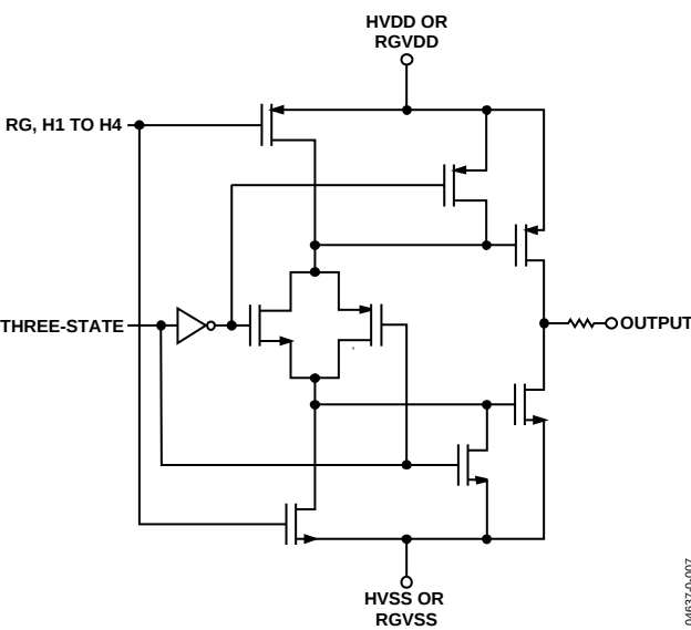
Figure 8. H1 to H4, RG Drivers
