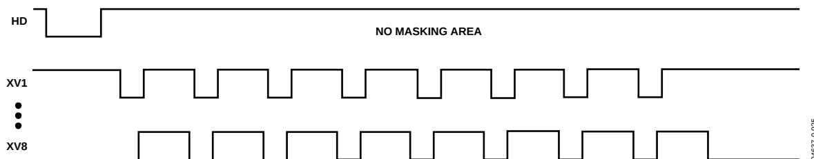
Figure 32. No Vertical Masking
