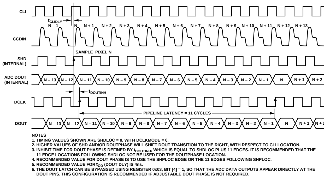
Figure 22. Digital Data Output Pipeline Delay
