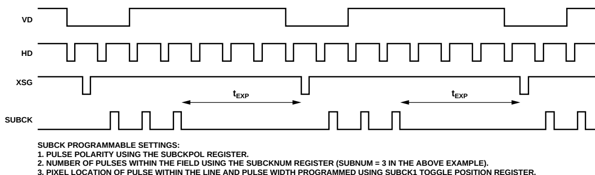
Figure 45. Normal Shutter Mode
