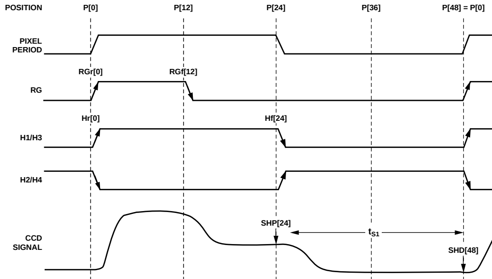
Figure 20. High Speed Timing Default Locations
