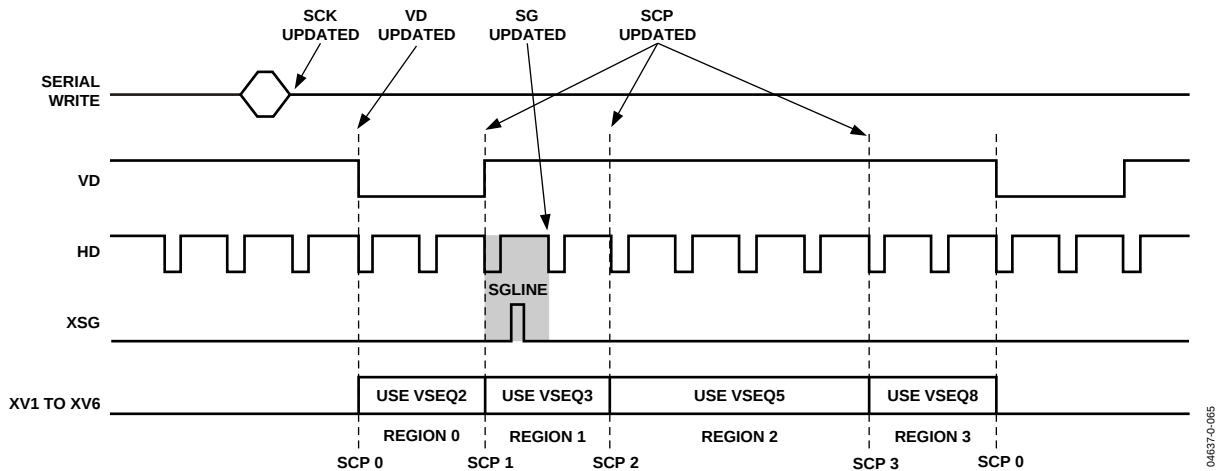
Figure 77. Register Update Locations (See Table 40 for Definitions)
