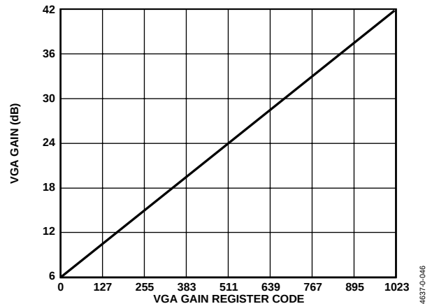
Figure 56. VGA Gain Curve
