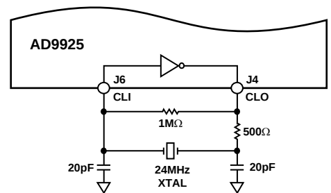
Figure 72. Crystal Driver Application
