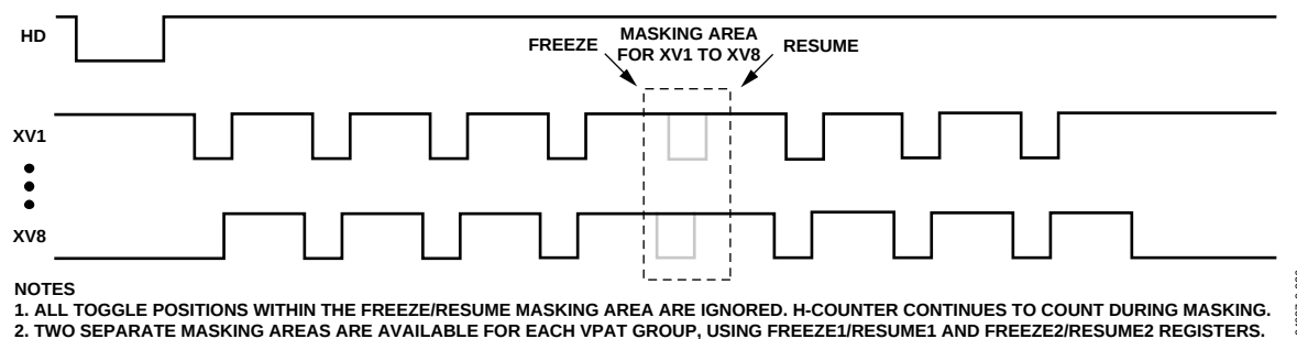
Figure 33. Vertical Masking Using the FREEZE/RESUME Registers
