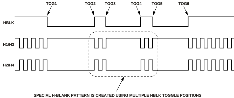
Figure 26. Generating Special HBLK Patterns
