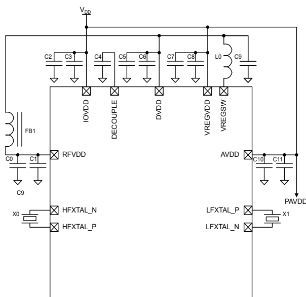
Figure 5.3. EFR32MG1 Typical Application Circuit: Configuration with DC-DC Coverter (PAVDD from VDD)
