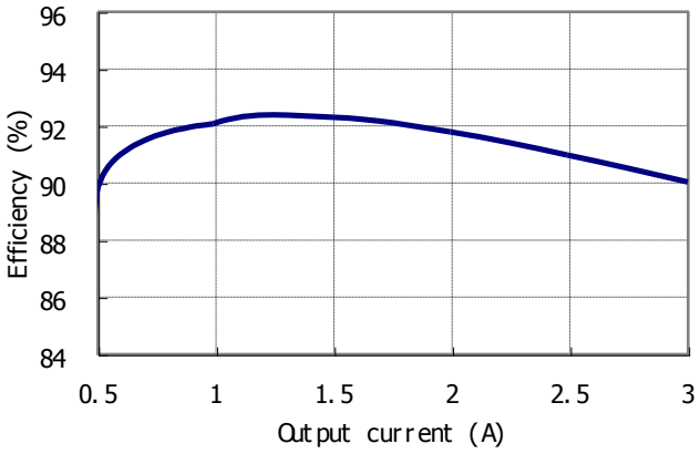
Figure 2: Converter efficiency vs. output current (5Vin/2.5Vout)
