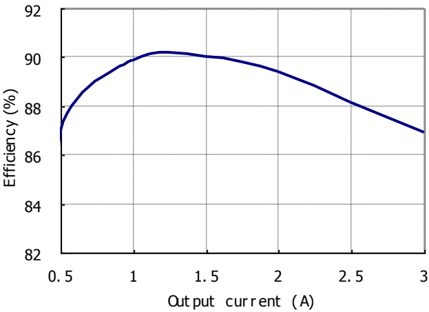
Figure 3: Converter efficiency vs. output current (5Vin/1.8Vout)
