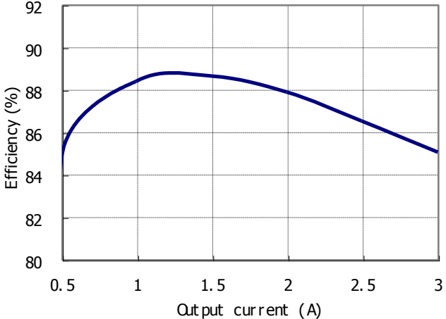
Figure 4: Converter efficiency vs. output current (5Vin/1.5Vout)
