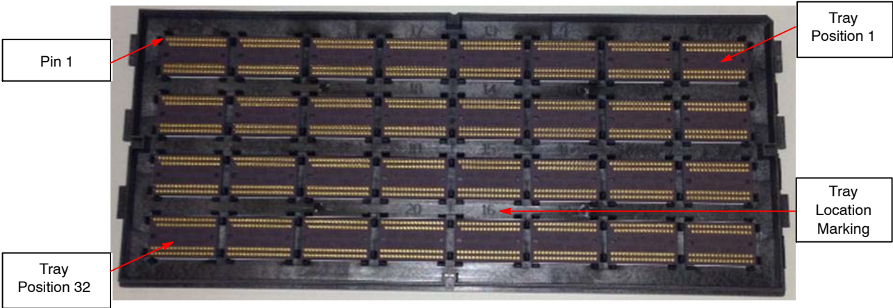
Figure 34. Tray Pin-Up View
