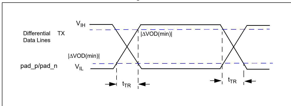
Figure 11. Rise/fall time
