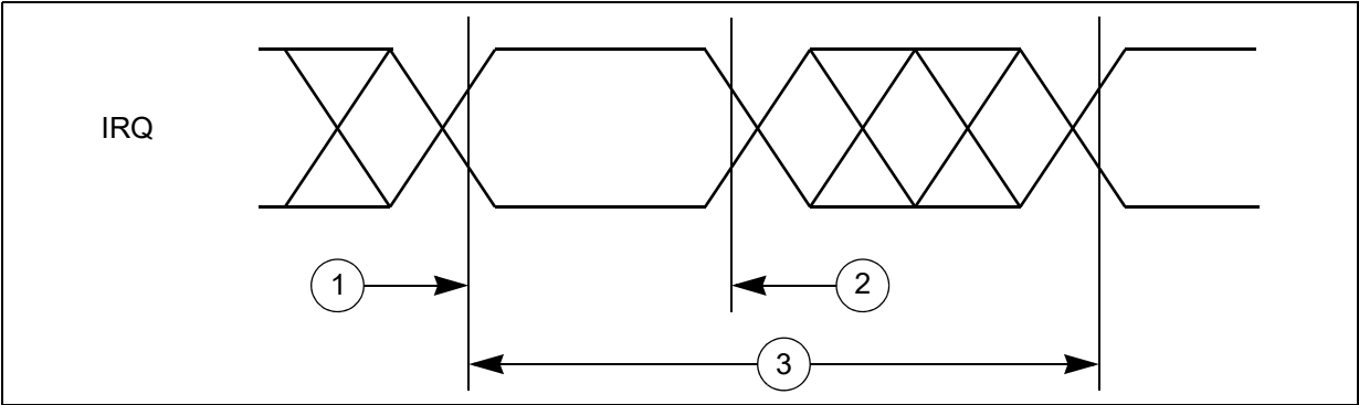
Figure 24. External interrupt timing
