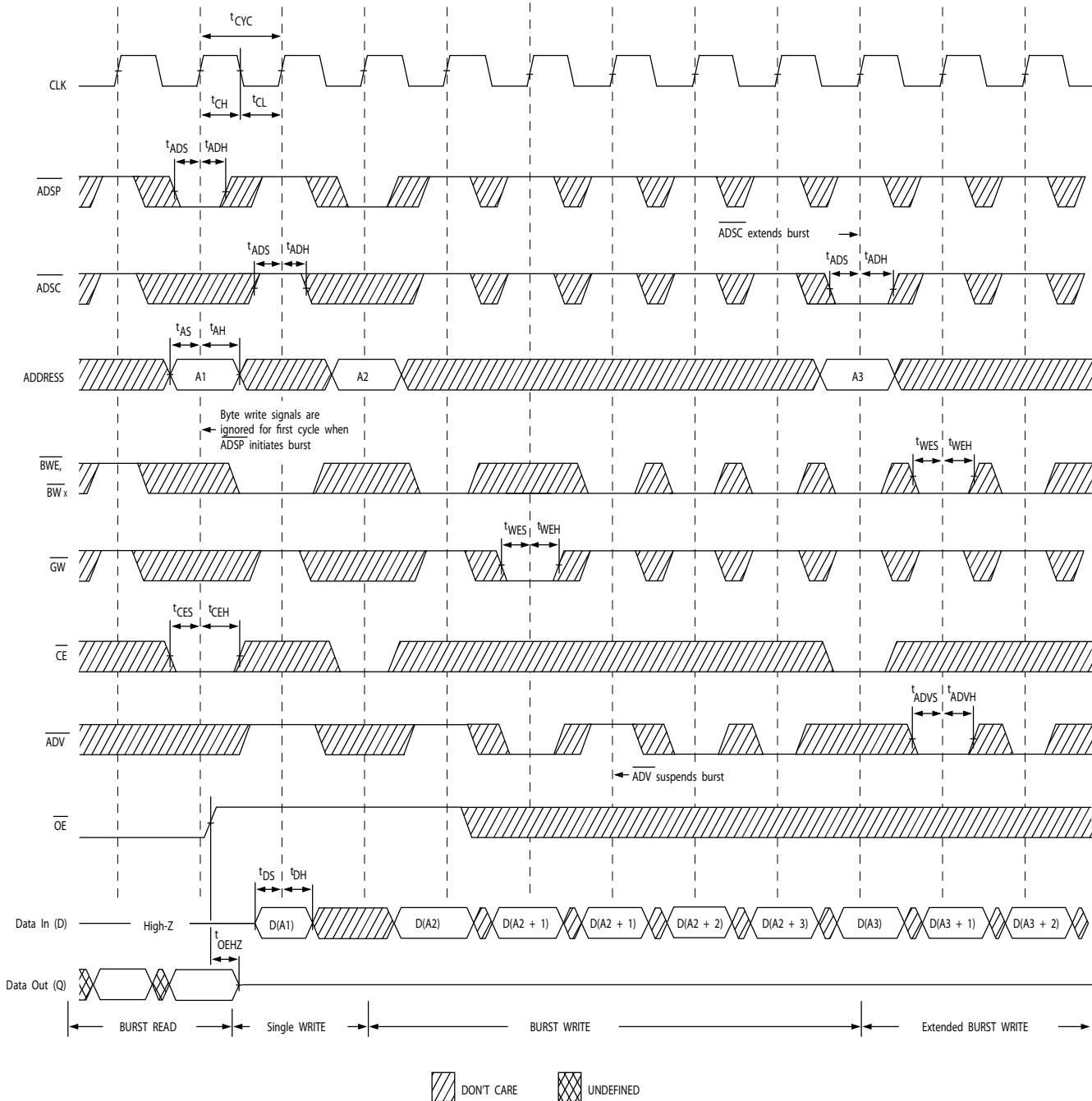
Figure 7. Write Cycle Timing [23, 24]
