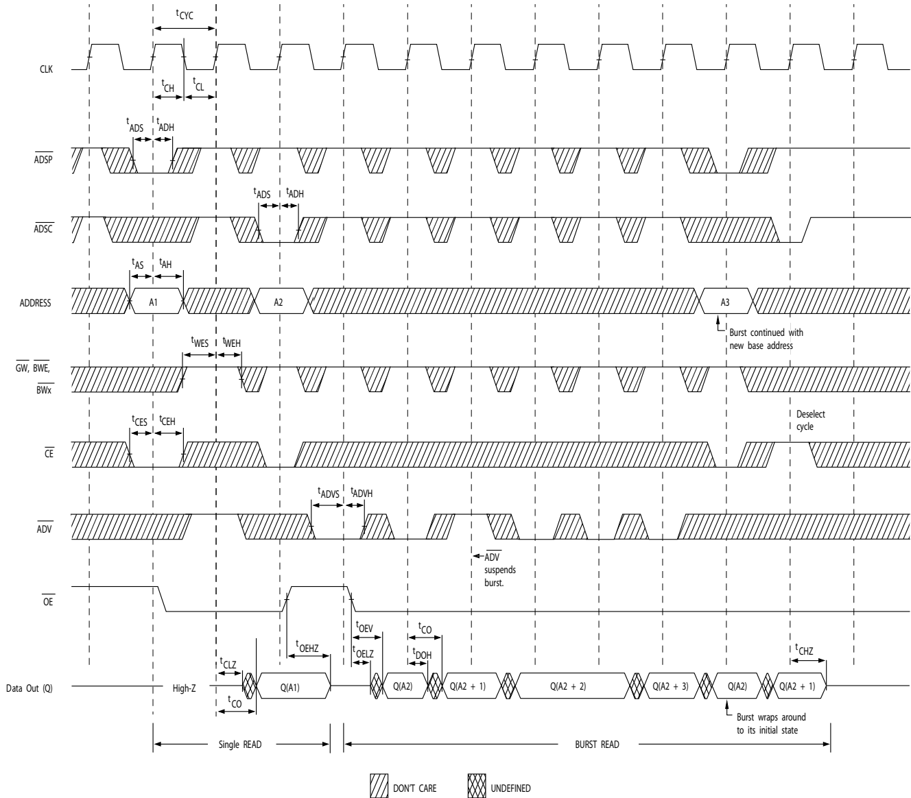
Figure 6. Read Cycle Timing [23]
