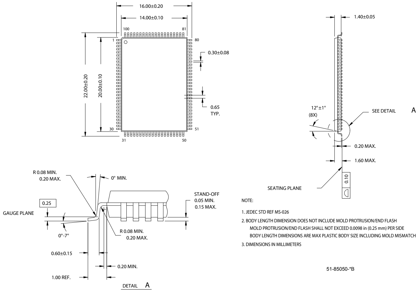
Figure 10. 100-Pin Thin Plastic Quad Flatpack (14X20X1.4 mm)
