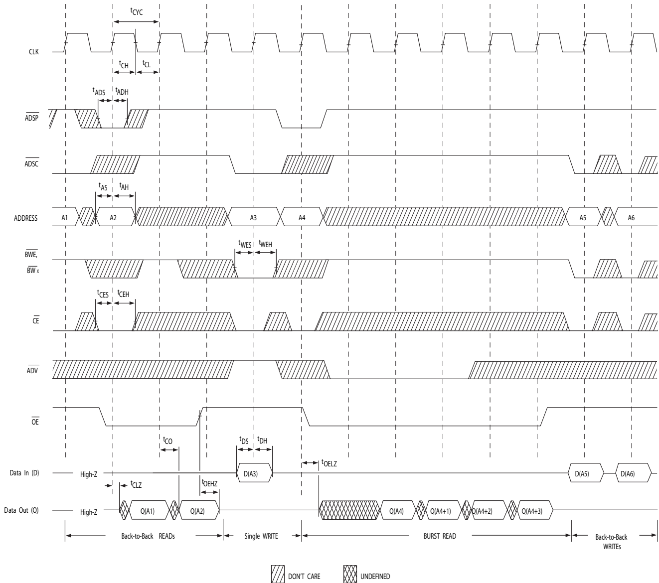
Figure 8. Read/Write Cycle Timing [23, 25, 26]
