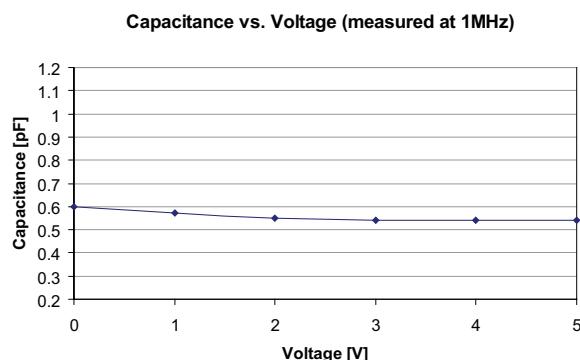
Figure 1. CM1214A Capacitance vs. Voltage
