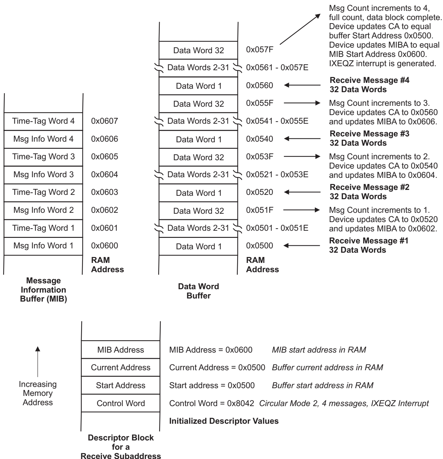
Figure 18. Circular Buffer Mode 2 Example for a Receive Subaddress
