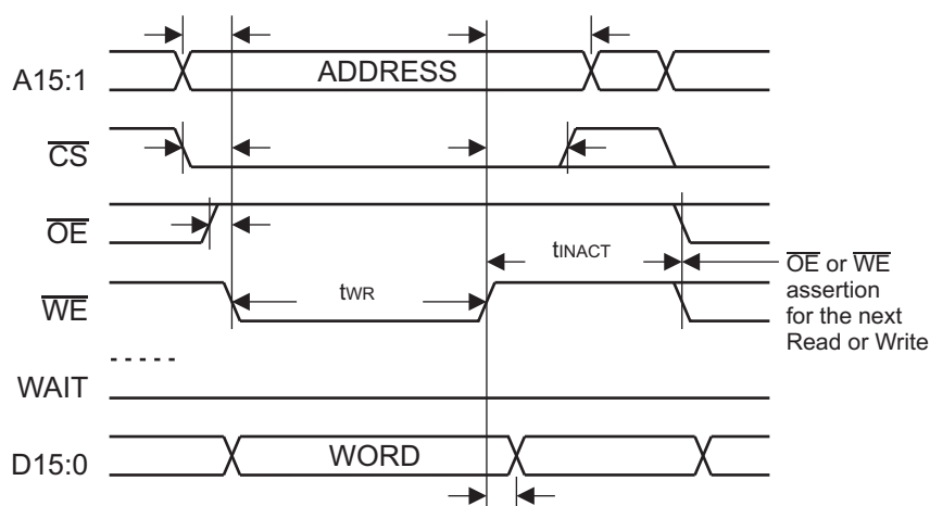
FIGURE 21. Register and RAM Write Operations for BTYPE = 1
