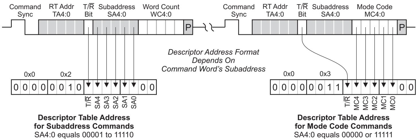
FIGURE 10. Deriving a Descriptor Table Control Word Address From Command Word
