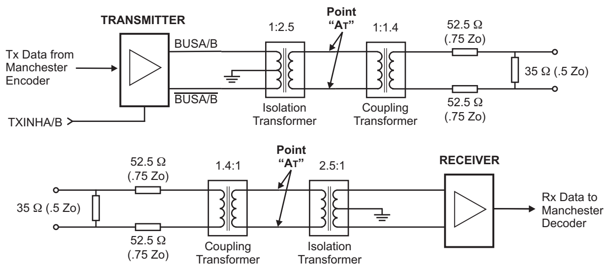
Figure 26. Transformer Coupled Test Circuits
