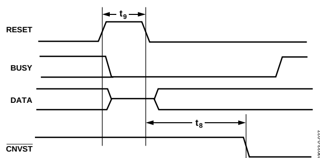
Figure 34. RESET Timing
