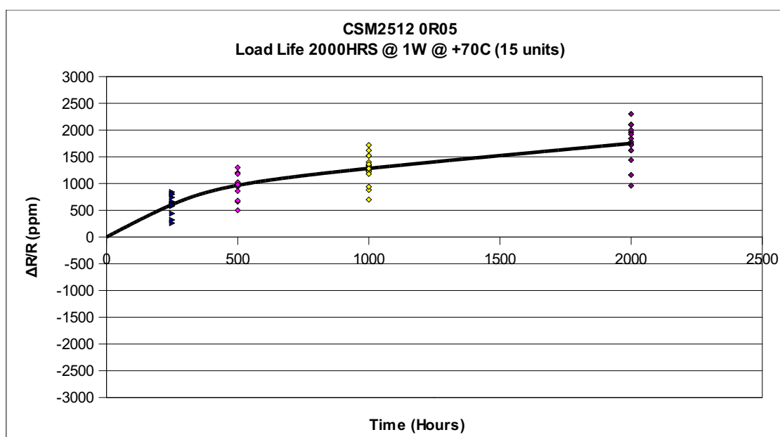
FIGURE 3 - LOAD LIFE RESULTS OF CSM2512
