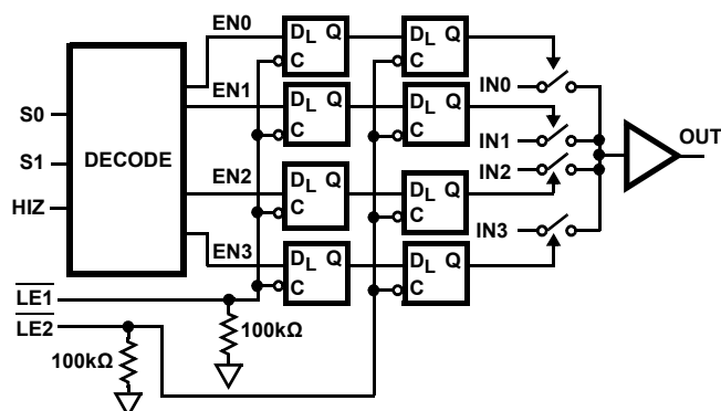
FIGURE 1. FUNCTIONAL DIAGRAM
