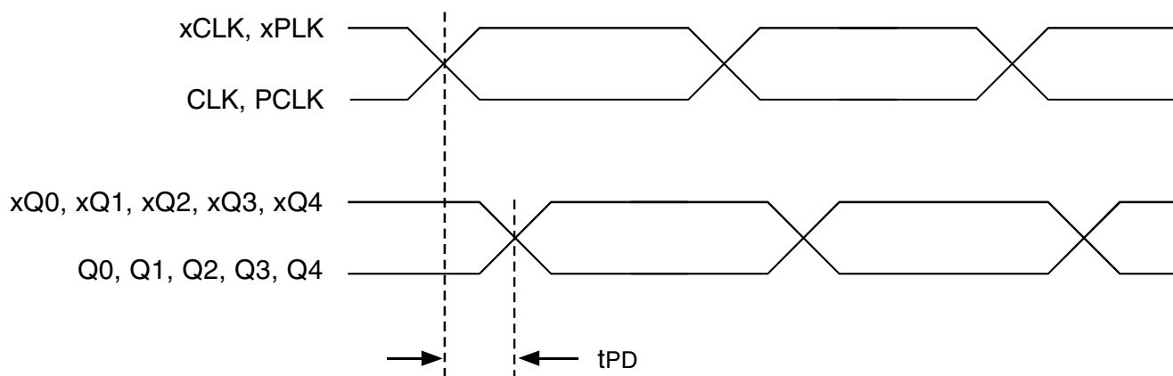
Propagation Delay
