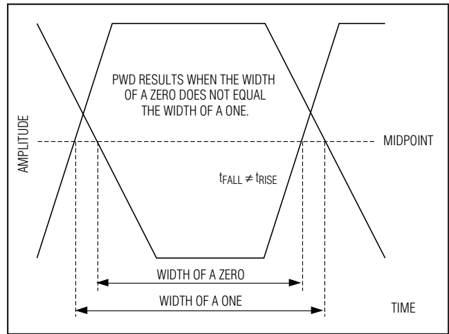
Figure 11. Pulse-Width Distortion
