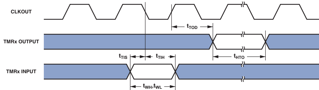
Figure 31. Timer PWM_OUT Cycle Timing
