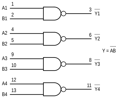
LOGIC DIAGRAM
