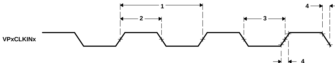
Figure 5-53. Video Port Display VPxCLKINx Timing
