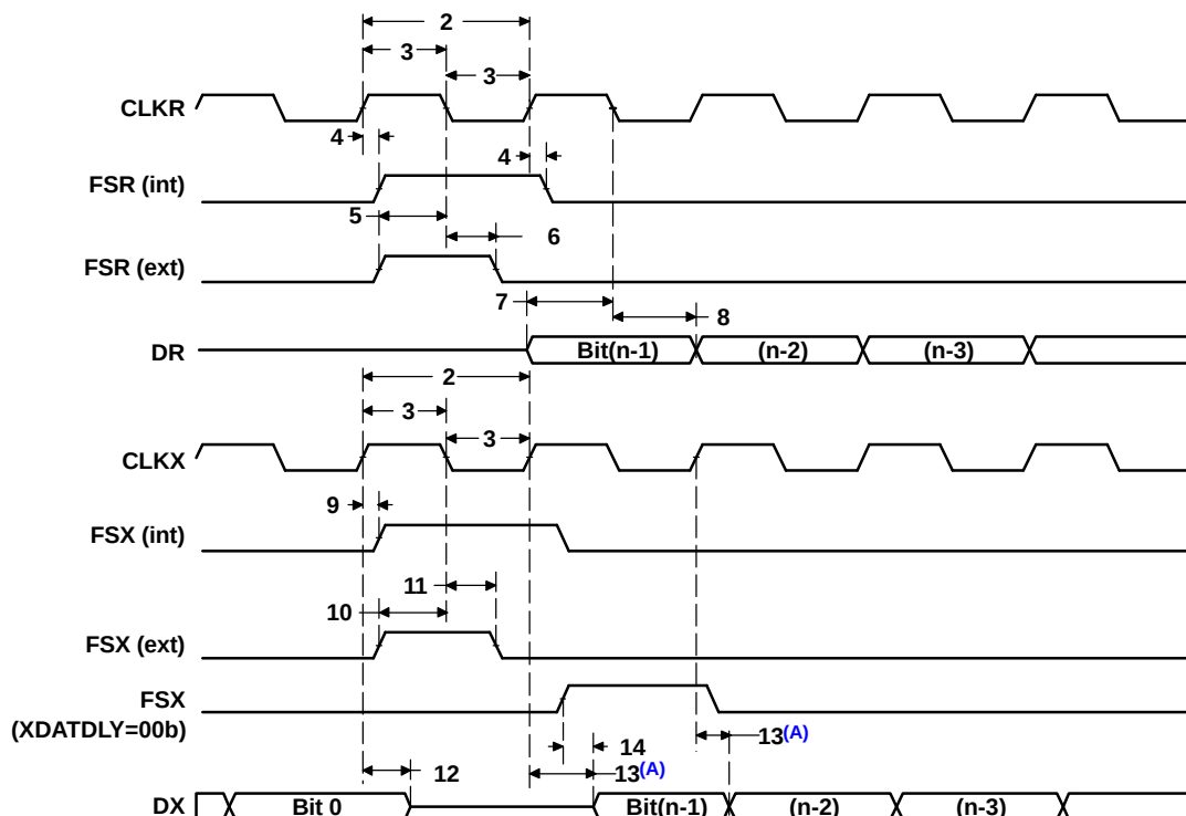
Figure 5-46. McBSP Timing
