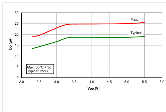
FIGURE 28-12: IDD, LFINTOSC Mode, Fosc = 31 kHz, PIC16F1574/5/8/9 Only.
