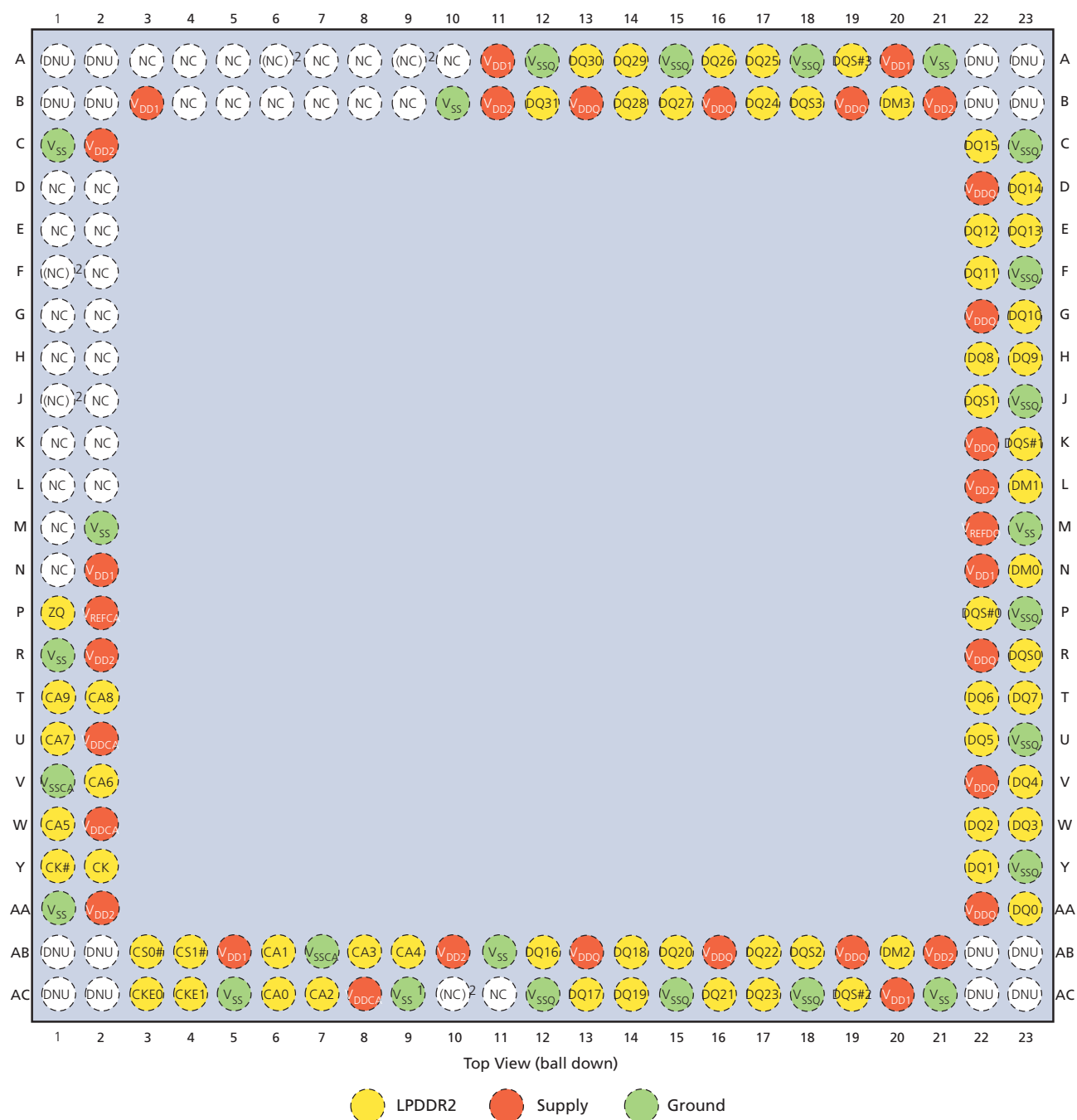
Figure 8: 168-Ball WFBGA – 12mm x 12mm
