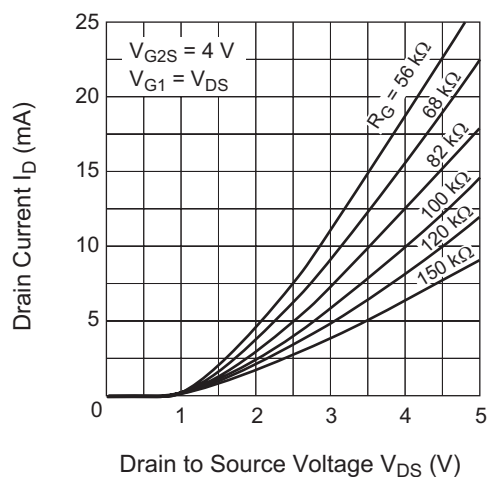
Typical Output Characteristics (FET2)
