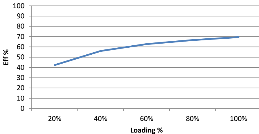
AM1DR-1215SZ Efficiency vs. Loading
