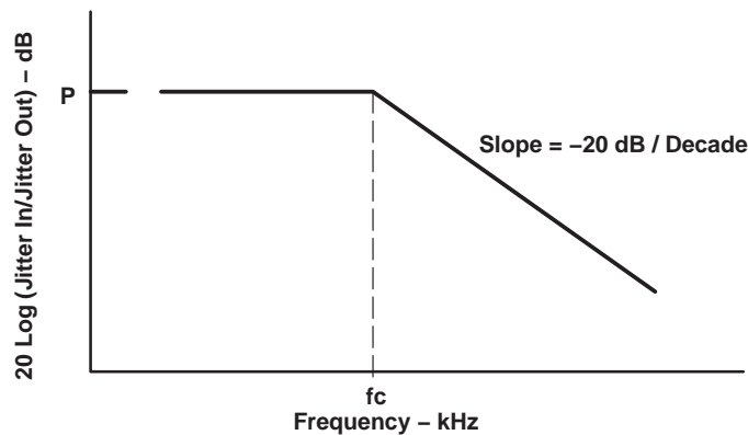
Figure 2. Jitter Transfer
