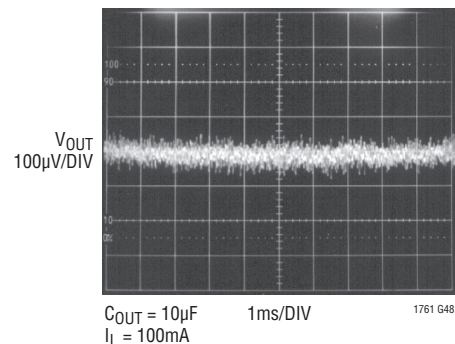
LT1761-5 10Hz to 100kHz Output Noise C_{\text{BYP}} = 0.01\mu\text{F}
