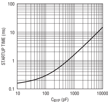
Startup Time
