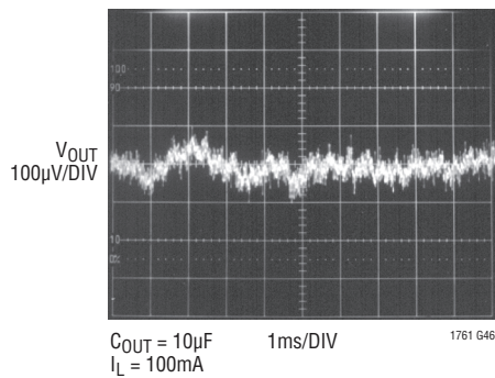
LT1761-5 10Hz to 100kHz Output Noise C_{\text{BYP}} = 1000\text{pF}
