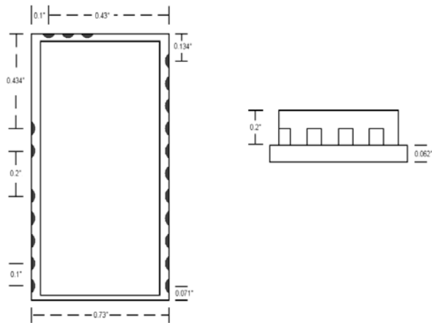
Figure 7: Mechanical Drawings for Wi.M868X-DP-R™
