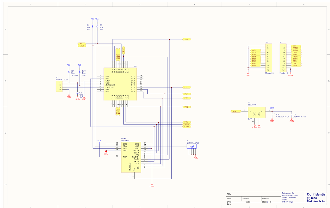
Figure 8: Evaluation Module Circuit
