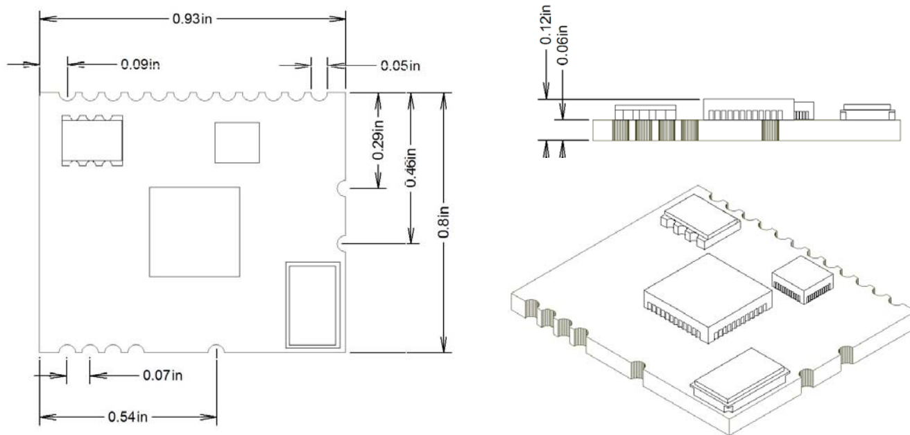
Figure 5: Module Mechanical Drawings for Wi.M868X-R™/ Wi.M868T-R™
