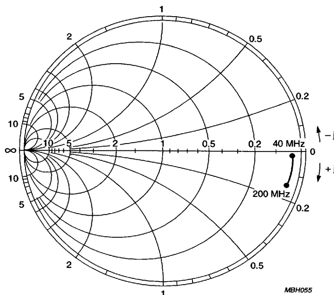
Fig.12 Input admittance ( S_{11} ) of the band A mixer input (40 to 200 MHz); Y_o = 20 \text{ mS} .
