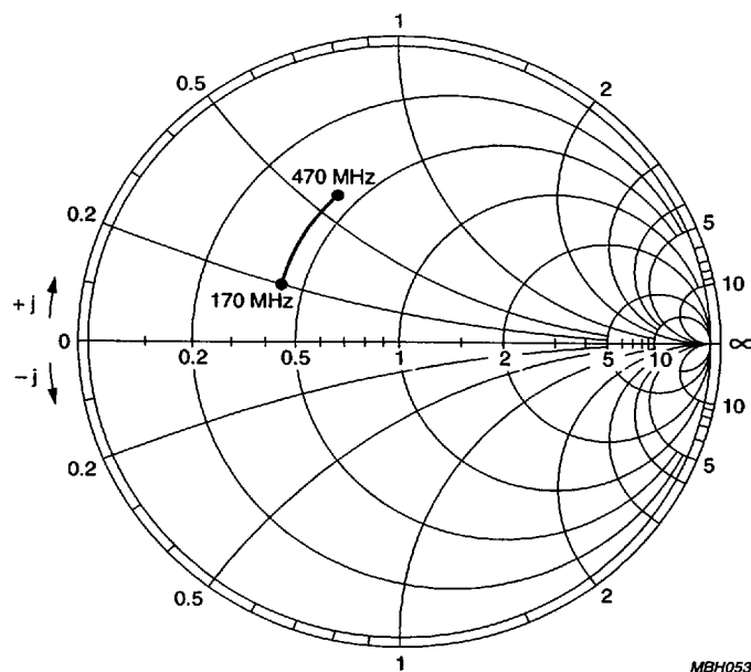
Fig.13 Input impedance ( S_{11} ) of the band B mixer input (170 to 470 MHz); Z_0 = 50 \Omega .
