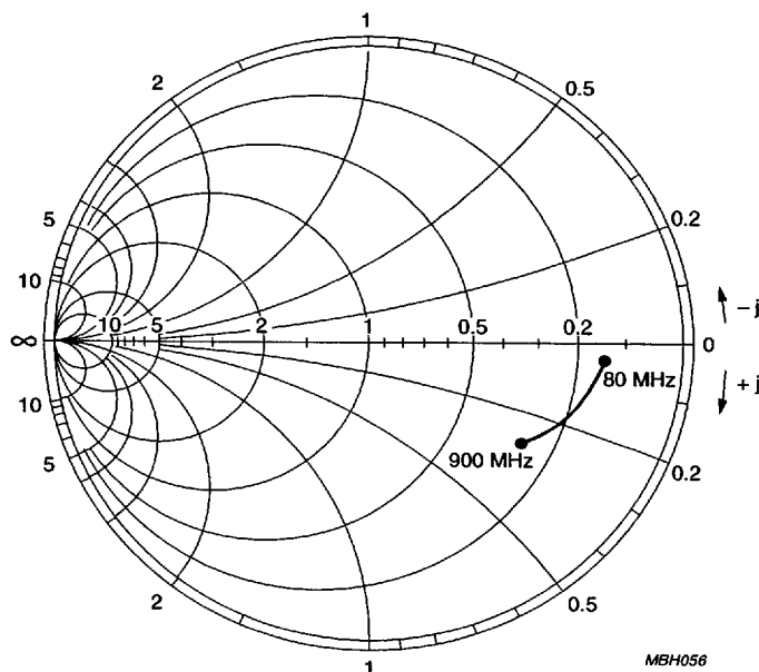
Fig.16 Input impedance ( S_{22} ) of the LO amplifier (80 to 900 MHz); Y_0 = 20 \text{ mS} .
