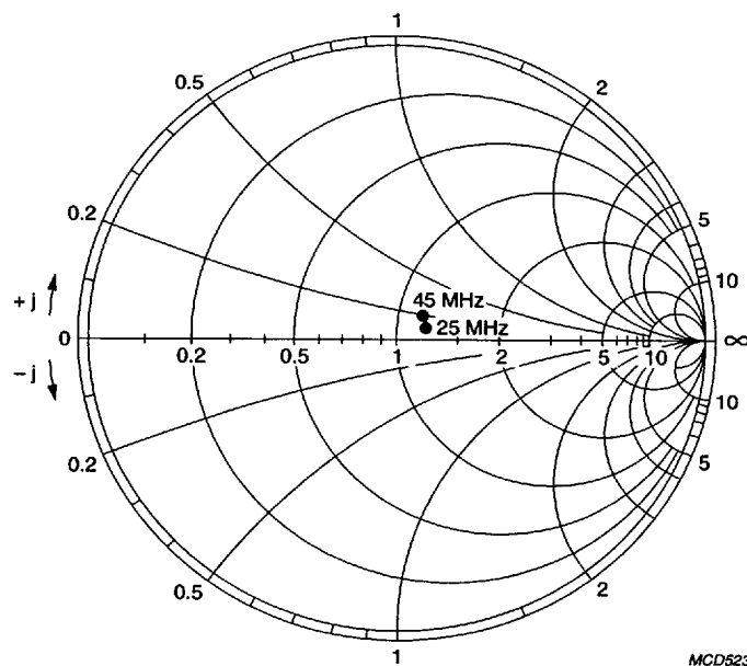
Fig.15 Input impedance ( S_{22} ) of the IF amplifier (25 to 45 MHz); Z_0 = 100 \Omega .
