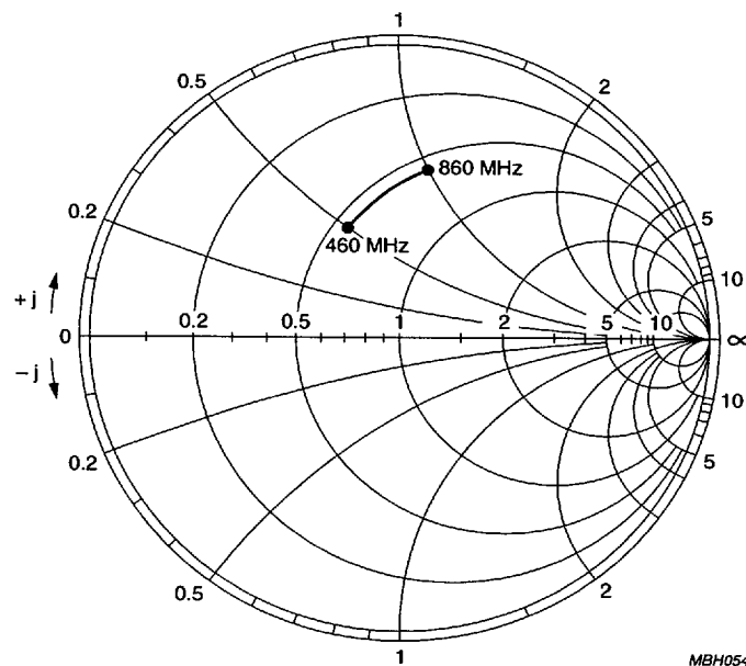
Fig.14 Input impedance ( S_{11} ) of the band C mixer input (460 to 860 MHz); Z_0 = 50 \Omega .
