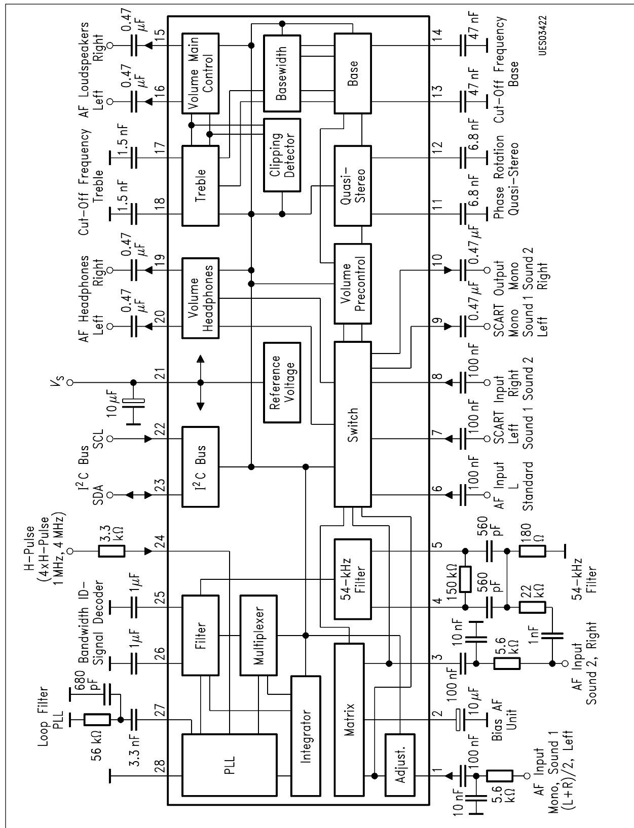
Application Circuit 2
