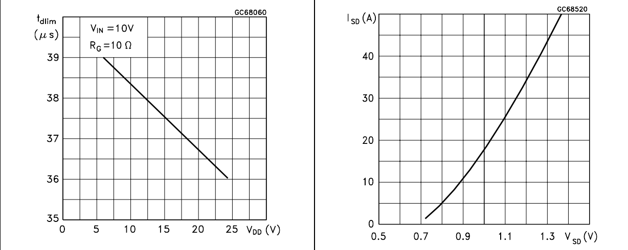
Figure 23. Step response current limit Figure 24. Source drain diode forward characteristics
