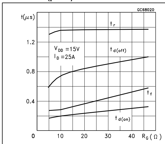
Figure 19. Switching time resistive load vs R_G (part 1)
