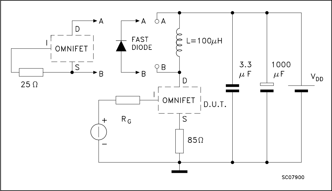
Figure 29. Test circuit for inductive load switching and diode recovery times
