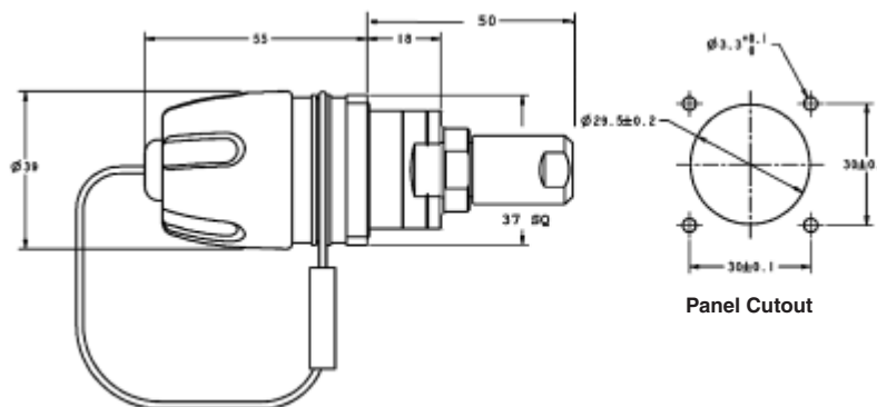
PRO BEAM Sr. Square Flange Mount Bulkhead with Standard Cable Adapter
