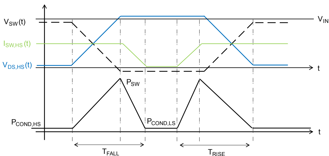
Figure 57. Switching losses
