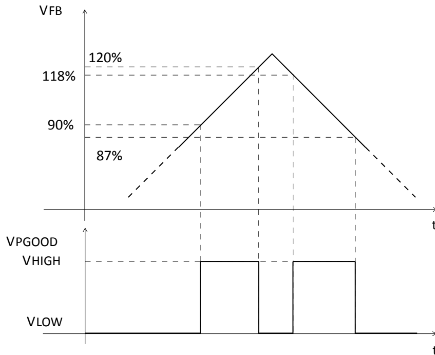
Figure 22. PGOOD thresholds
