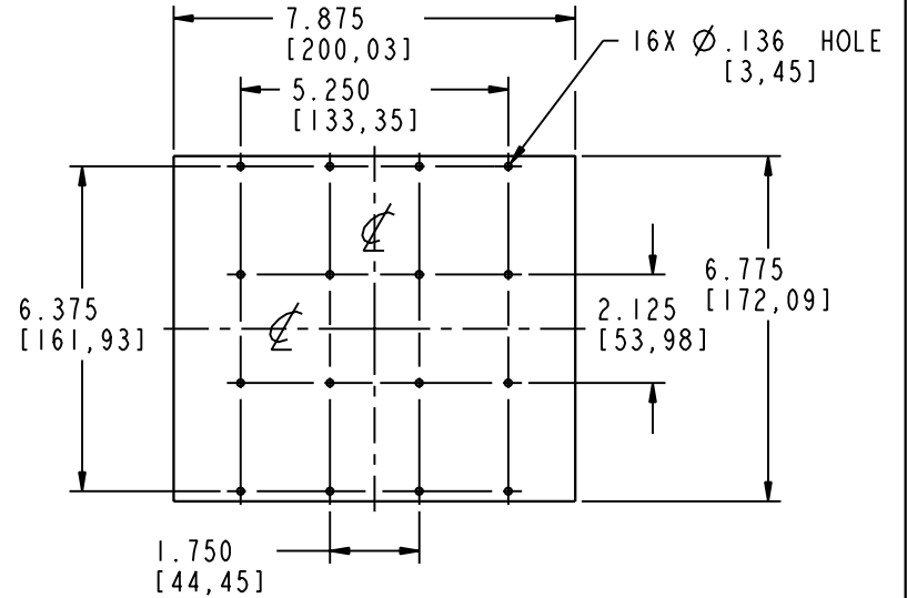
RECOMMENDED PC BOARD SIZE
