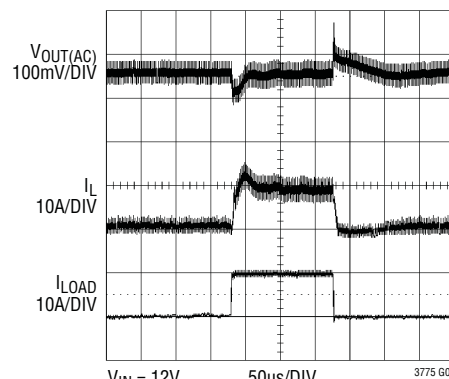
Load Step in Pulse-Skipping Mode
