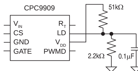
Figure 2 Soft-Start Circuit
