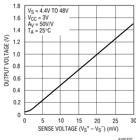
Figure 7. Expanded View of Output Voltage vs V_{SENSE} , A_V = 50V/V
